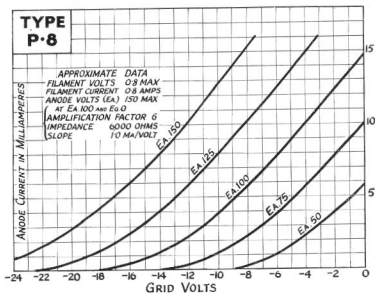
Characteristic Curve of average P.8 Valve.
